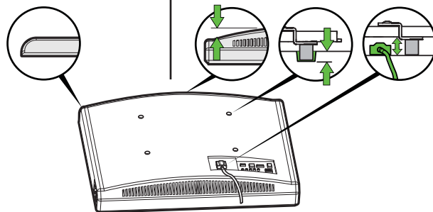
Flat Back
