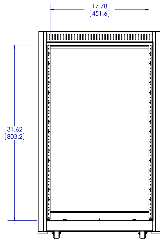
INTERNAL DIMENSIONS
